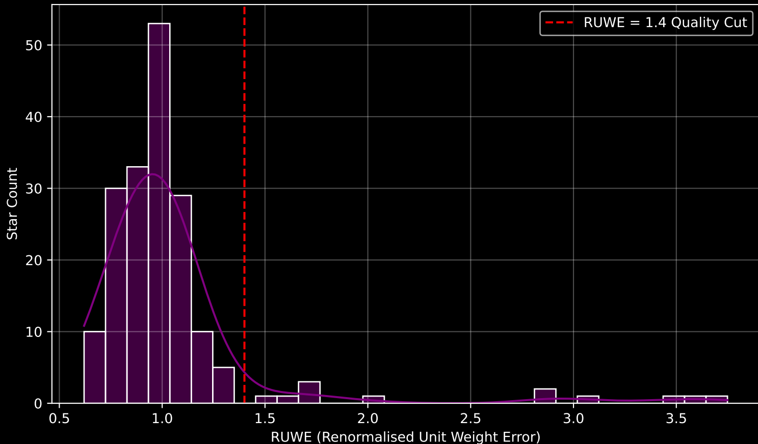
GAPOGEE DR17 Field [281-36-O] RUWE Distribution (n= 182)
