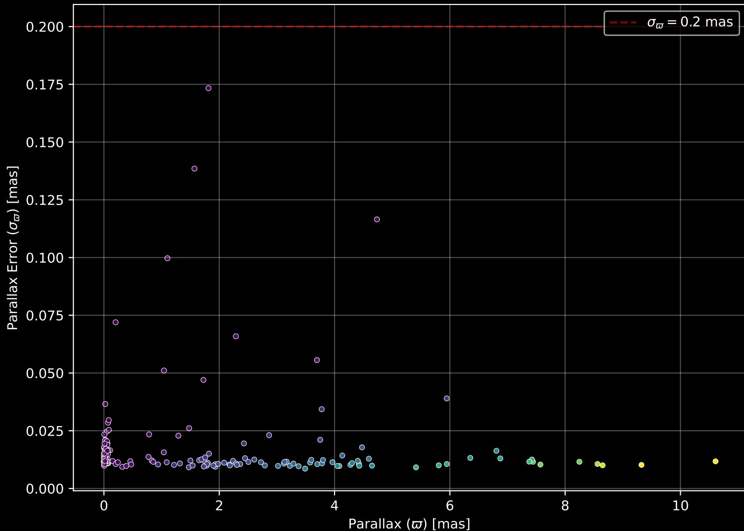
APOGEE DR17 Field: [281-36-O] Parallax Quality (n= 188)
