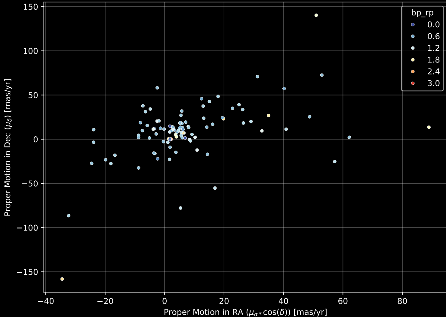
APOGEE DR17 Field: [281-36-O] Proper Motion Diagram (n= 188)
