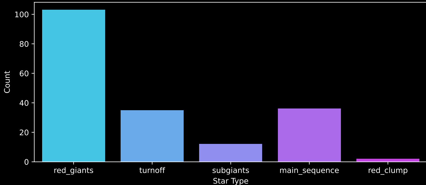
APOGEE DR17 Field: [281-36-O] Count plot of Star Type
